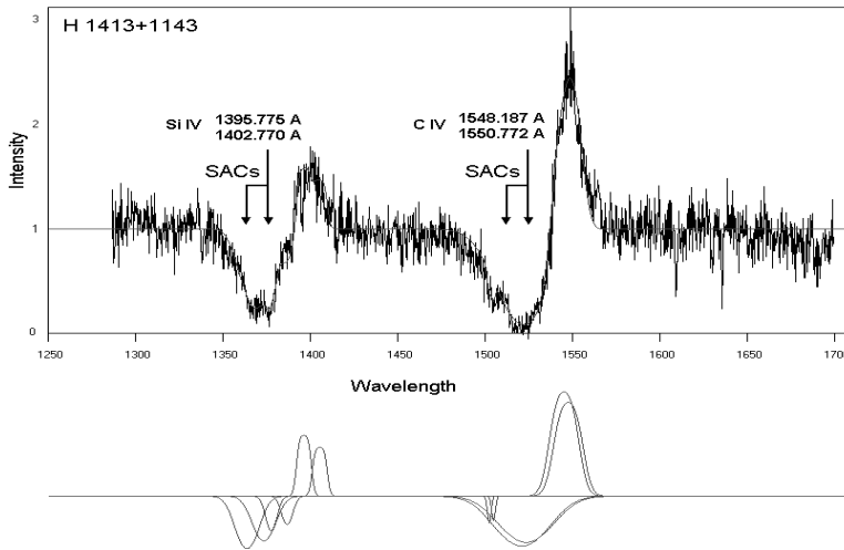
Figure 3 Fitting of the Si IV and C IV resonance lines of the AGN H 1413+1143, that present SACs with the proposed model. The SACs phenomenon is able to explain the observed shape.
