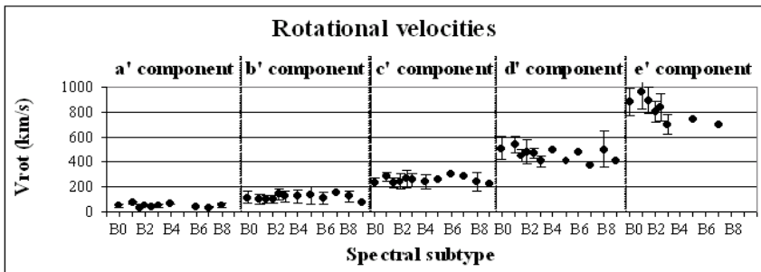
Figure 4. Mean rotational velocities of the independent density regions of matter which create the SACs of the Si IV resonance lines ( \lambda\lambda 1393.755, 1402.77 Å) as a function of the spectral subtype, in a sample of 68 Be stars.
