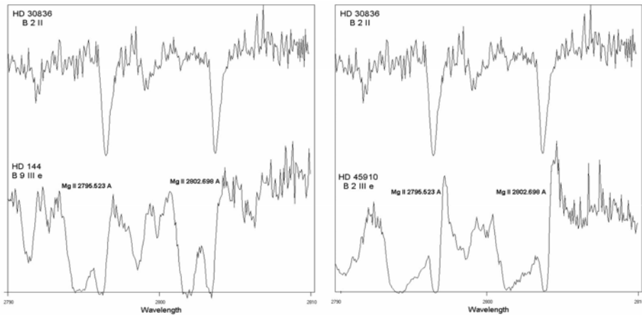
Figure. 1: Comparison of the Mg II resonance lines between the spectrum of a normal B star and the spectra of two active Be stars that present complex and peculiar spectral lines. As we can observe the Be stars present some absorption components that do not appear in the spectrum of the classical B star.
