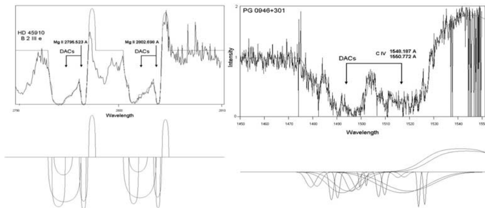
Figure 2: DACs phenomena in AGNs spectra: Similarity of DACs phenomenon in Be star's HD 45910 spectrum (Mg II doublet) with AGNs PG 0946+301 spectrum (C IV doublet). In the case of the C IV doublet, the two discrete features do not correspond to the two resonance lines, as the two members of the doublet have small difference in wavelength (1548.187 Å and 1550.772 Å) and they both lie at the right feature.
