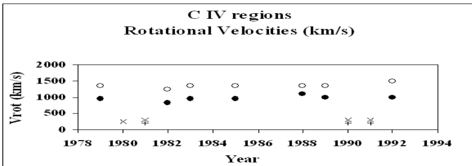
Figure 5 Variation of the rotational velocities of the C IV density regions of the Oe star HD 149757, as a function of time.
